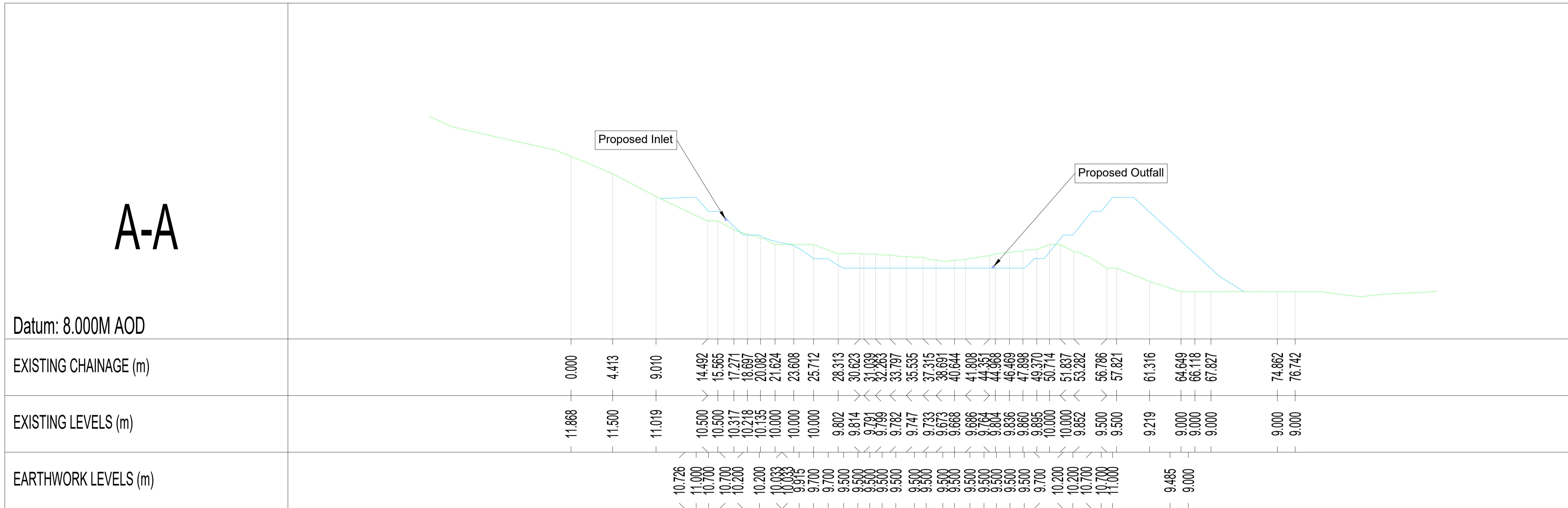
Section A-A: Scale @A1 Horizontal 1:250 / Vertical 1:50 @A3 Horizontal 1:500 / Vertical 1:100
